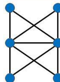
Graph H_2
