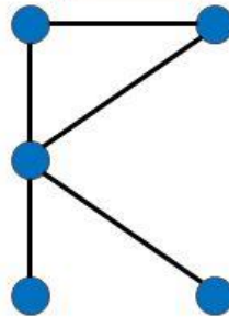
Graph H_1
