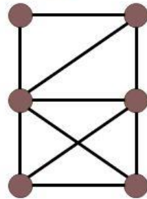
Graph G
